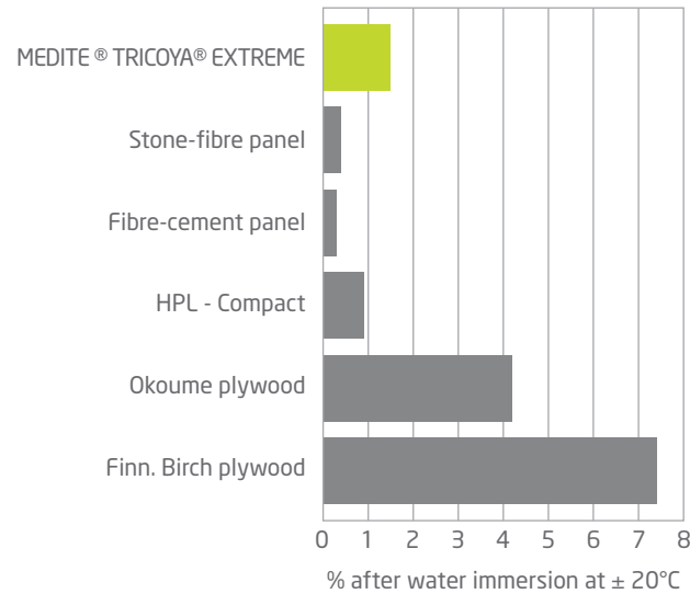
Thickness swell
